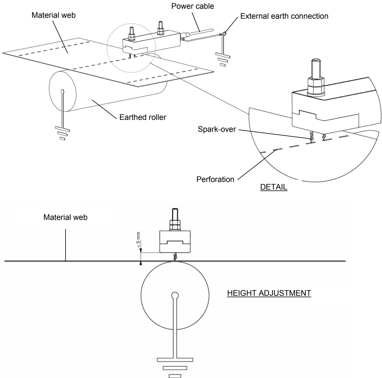
Figure 3, Perfomaster installation
