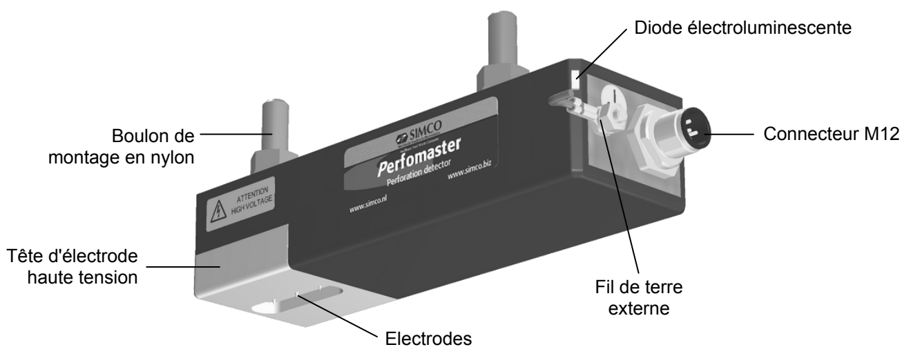
Figure 1, Perfomaster
