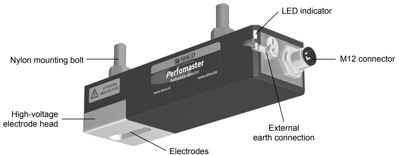
Figure 1, Perfomaster
