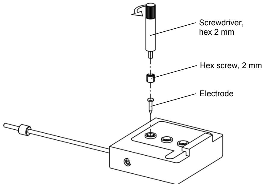
Figure 7, replacing electrodes
