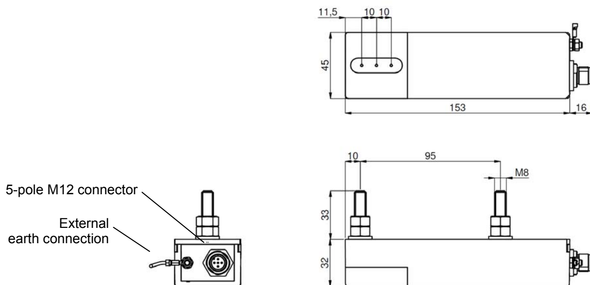
Figure 2, Perfomaster dimensions
