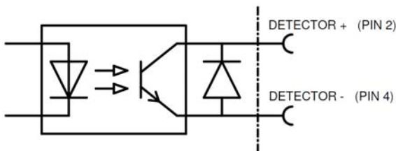
Figure 4, Perfomaster connections
