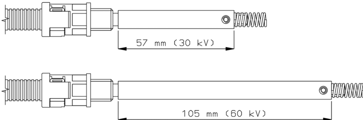
Figure 1: 30 kV and 60 kV HV connectors
